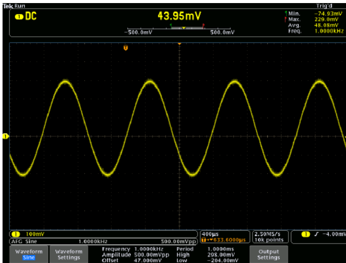
A DC measurement value is shown with a five second variation along with minimum, maximum, and average voltage values. The frequency of the waveform is also shown.
