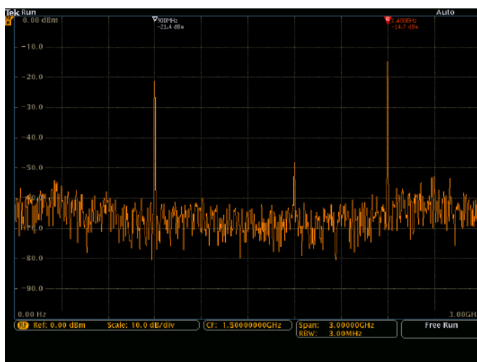
Spectral display of a bursted communication both into a device through Zigbee at 900 MHz and out of the device through Bluetooth at 2.4 GHz, captured with a single acquisition.
